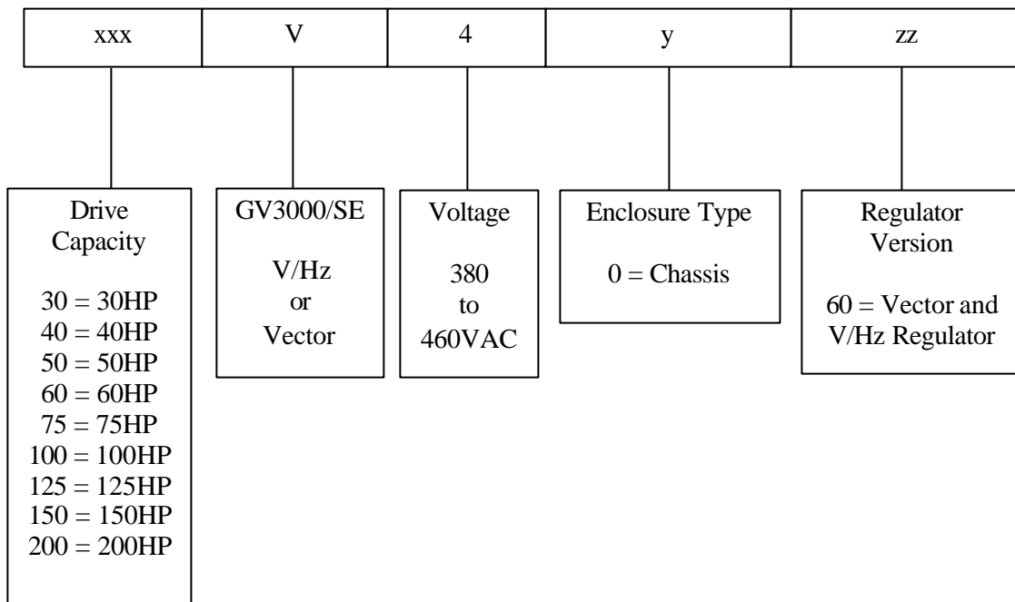
Fig.A Drive Configuration
