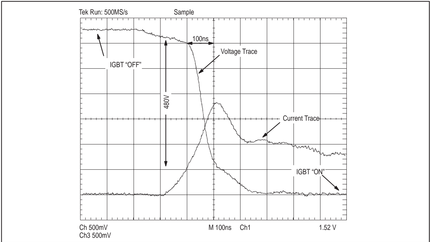
Figures 5. Oscilloscope trace.
