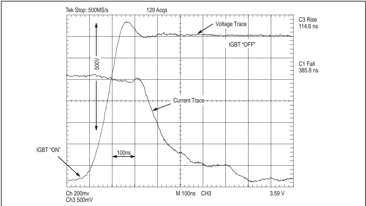
Figures 6. Oscilloscope trace.
