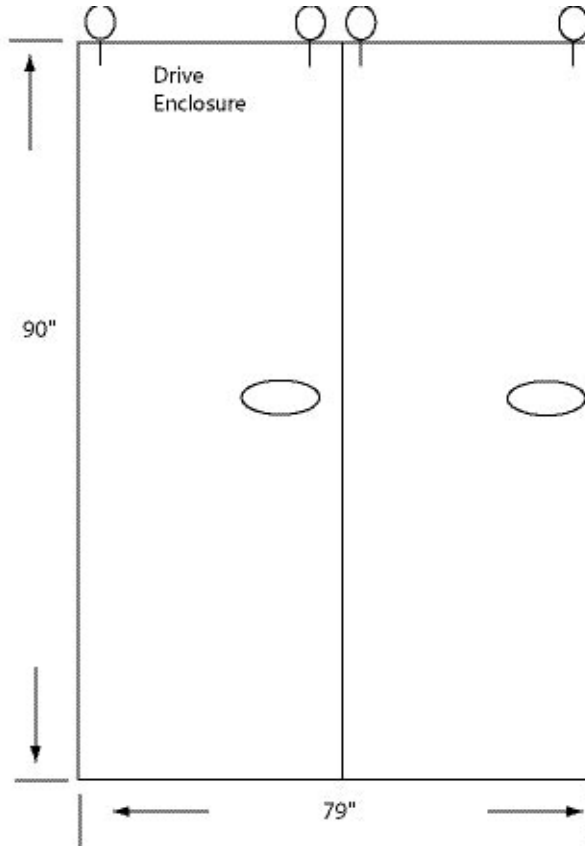
120 L Basic Dimensions
